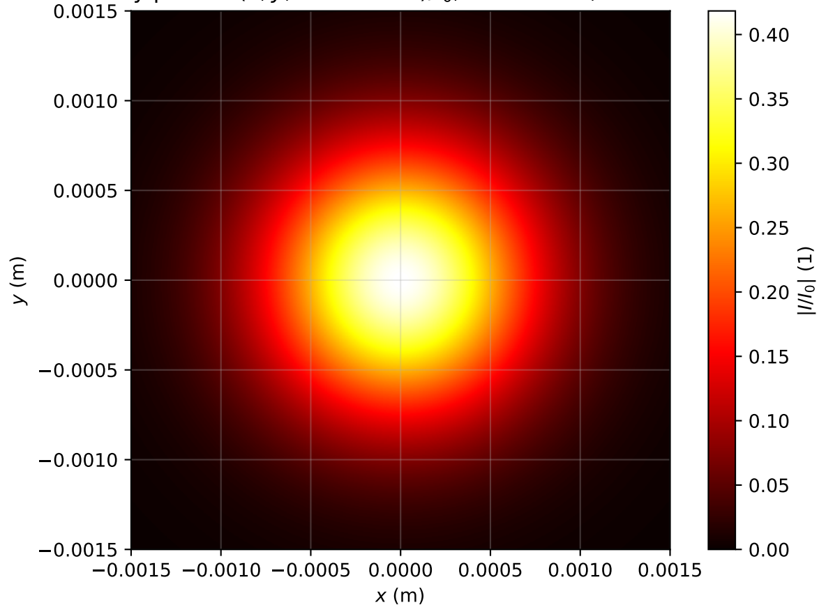
Intensity profile I(x, y, z = 3.025m)/I_0 , P_{in}=0.3P_{cr} , artificial time
